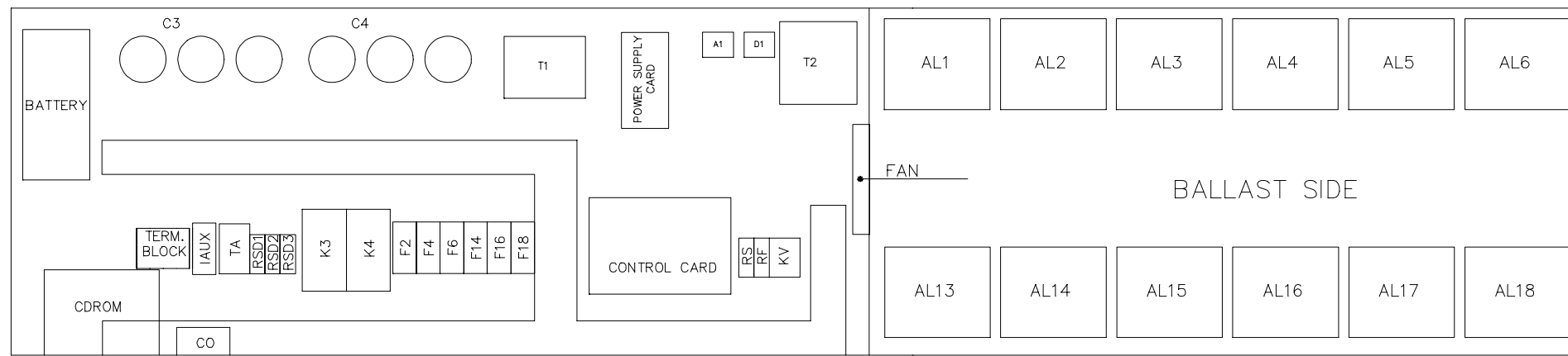
FRONT VIEW
