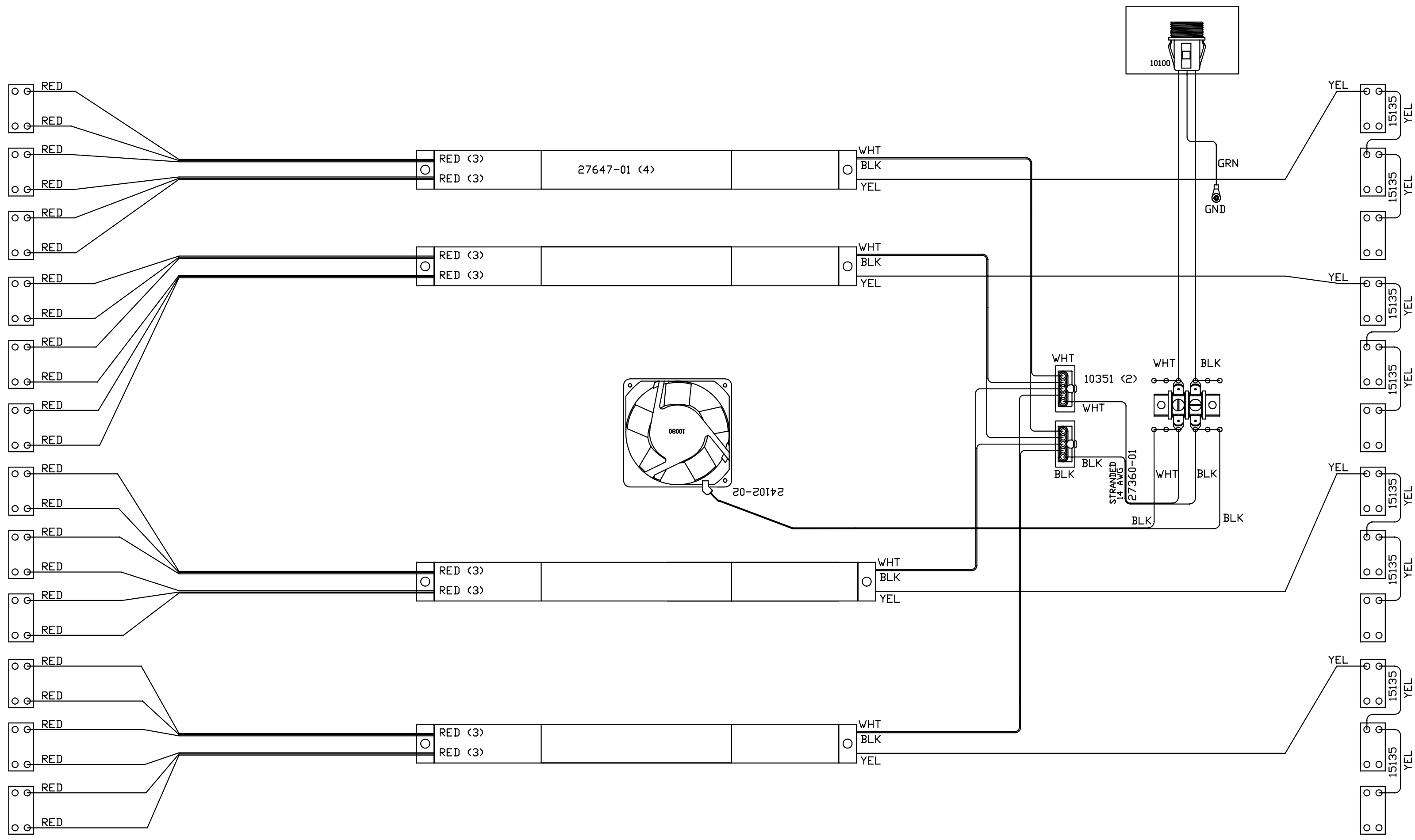
27520-01, REV A BENCH, 12 LAMP 120 VAC FRONT OF BED
