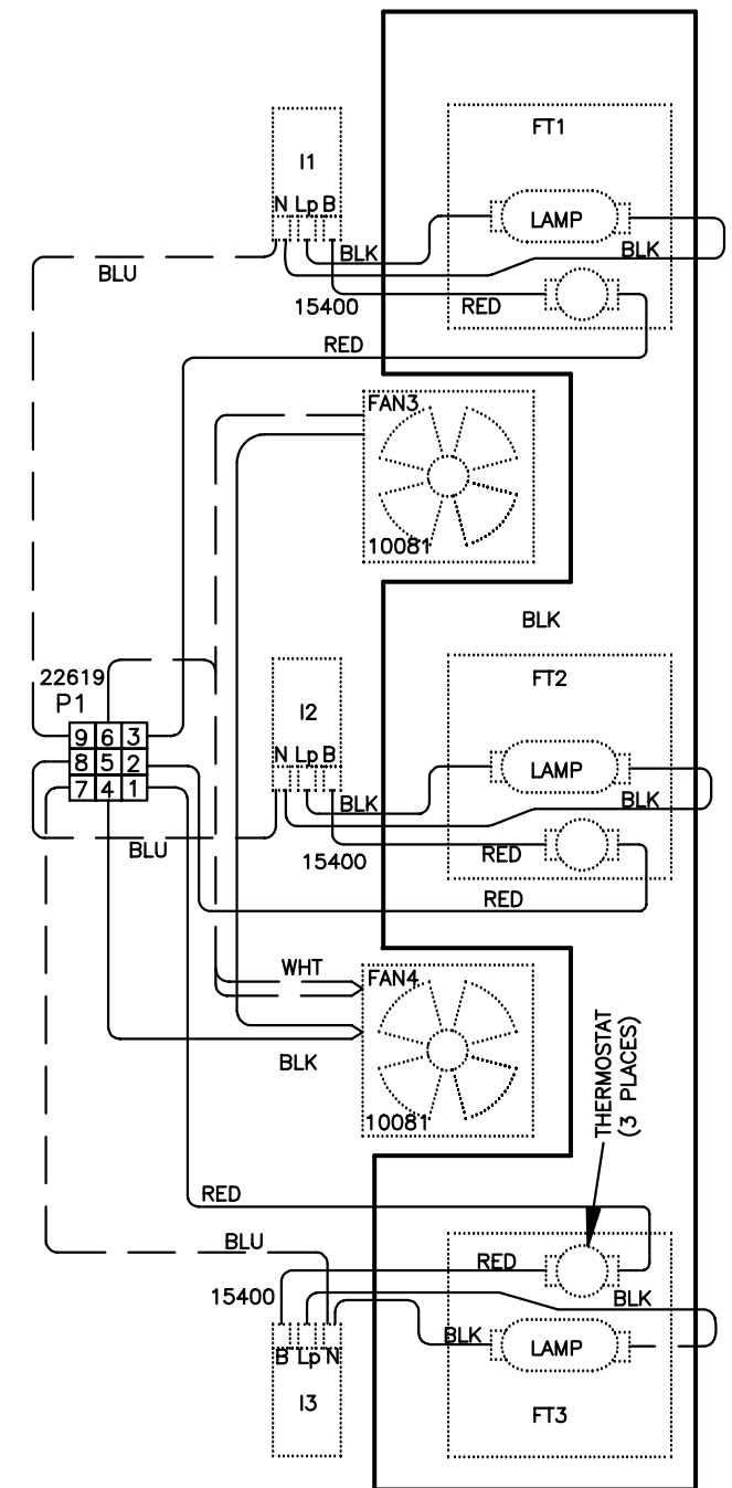
FACE TANNER SHROUD WIRE DIAGRAM
