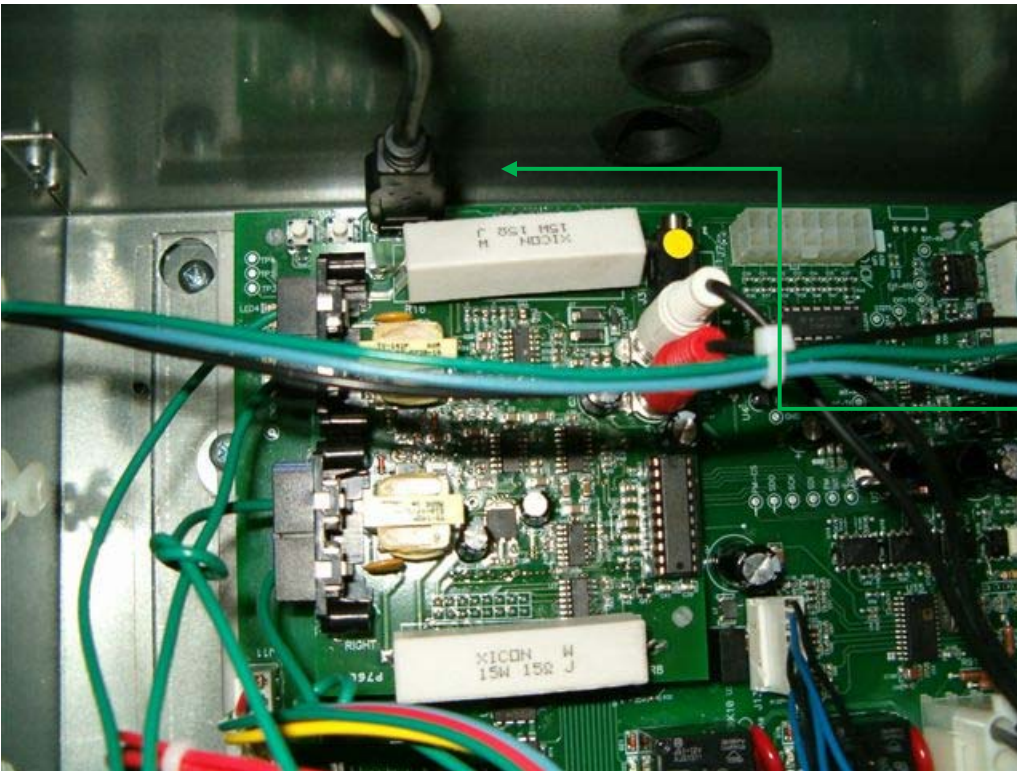
View from inside the timer box. First remove cover from timer box, and then plug the cable in here.
